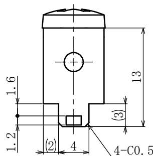
A 詳細図 (4/1) Detailed view A (4/1)
