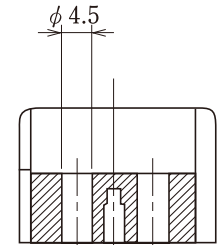
A-A'断面/Section
