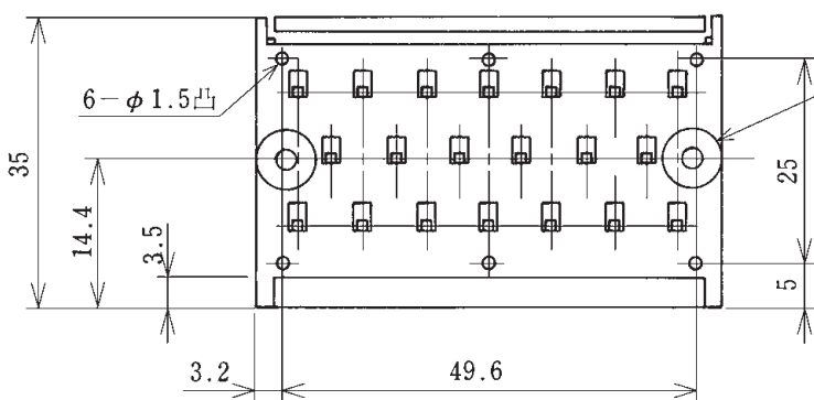
A 矢視図 Drawing of view A
