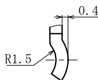
A 詳細図(4/1) Detailed view A(4/1)
