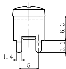
A 詳細図(4/1) Detailed view A(4/1)
