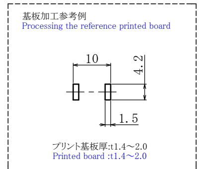
A詳細図(4/1) Detaild view A(4/1)
