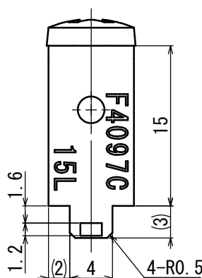
A詳細図 (4/1) Detailed view A (4/1)
