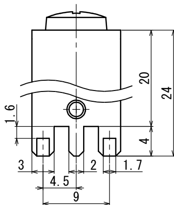
A詳細図 (4/1) Drawing view A(4/1)
